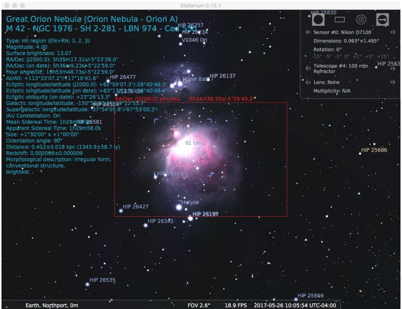
Orion Nebula - APS-C, 900 mm FL Telescope
