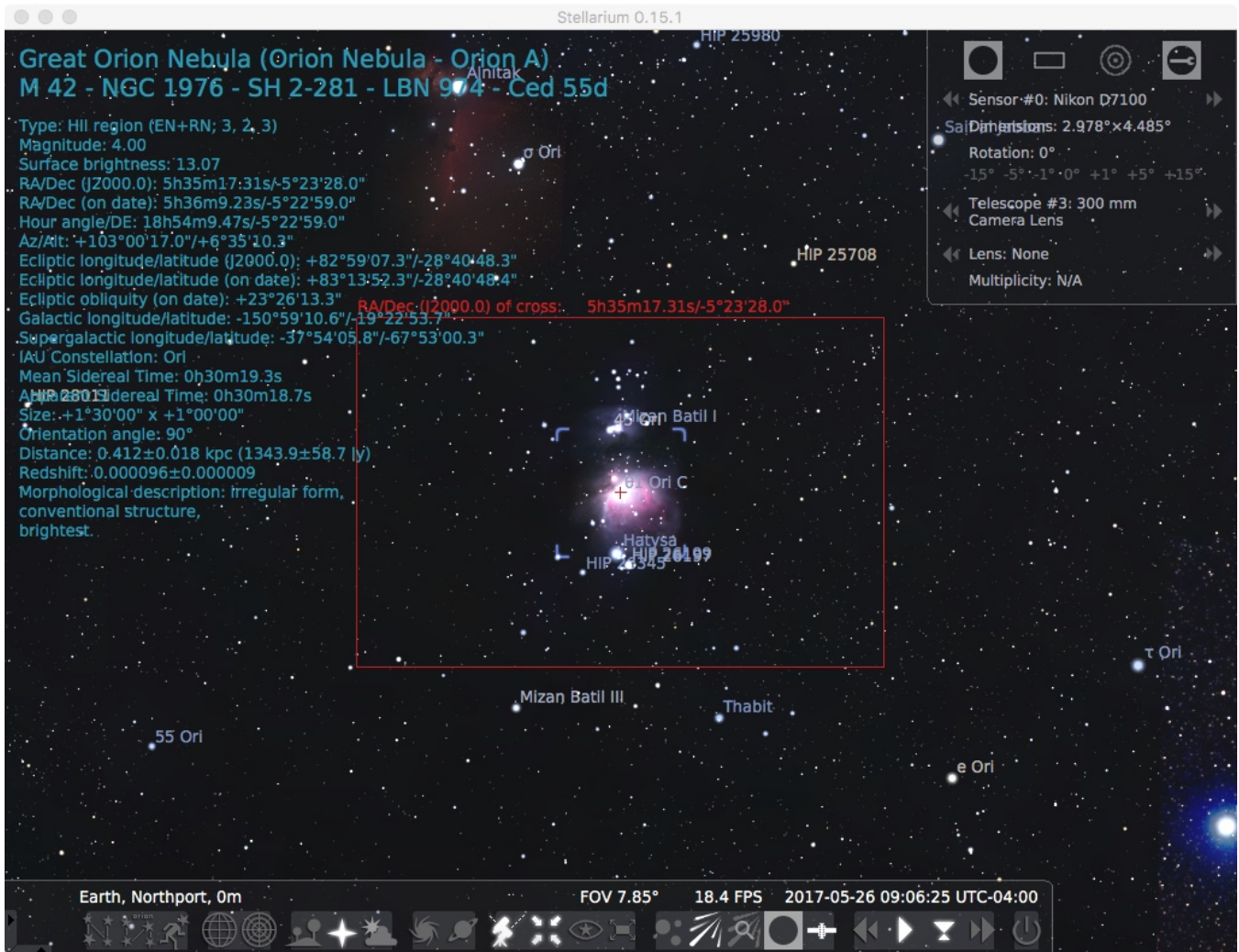
Orion Nebula - APS-C, 300 mm FL Lens
