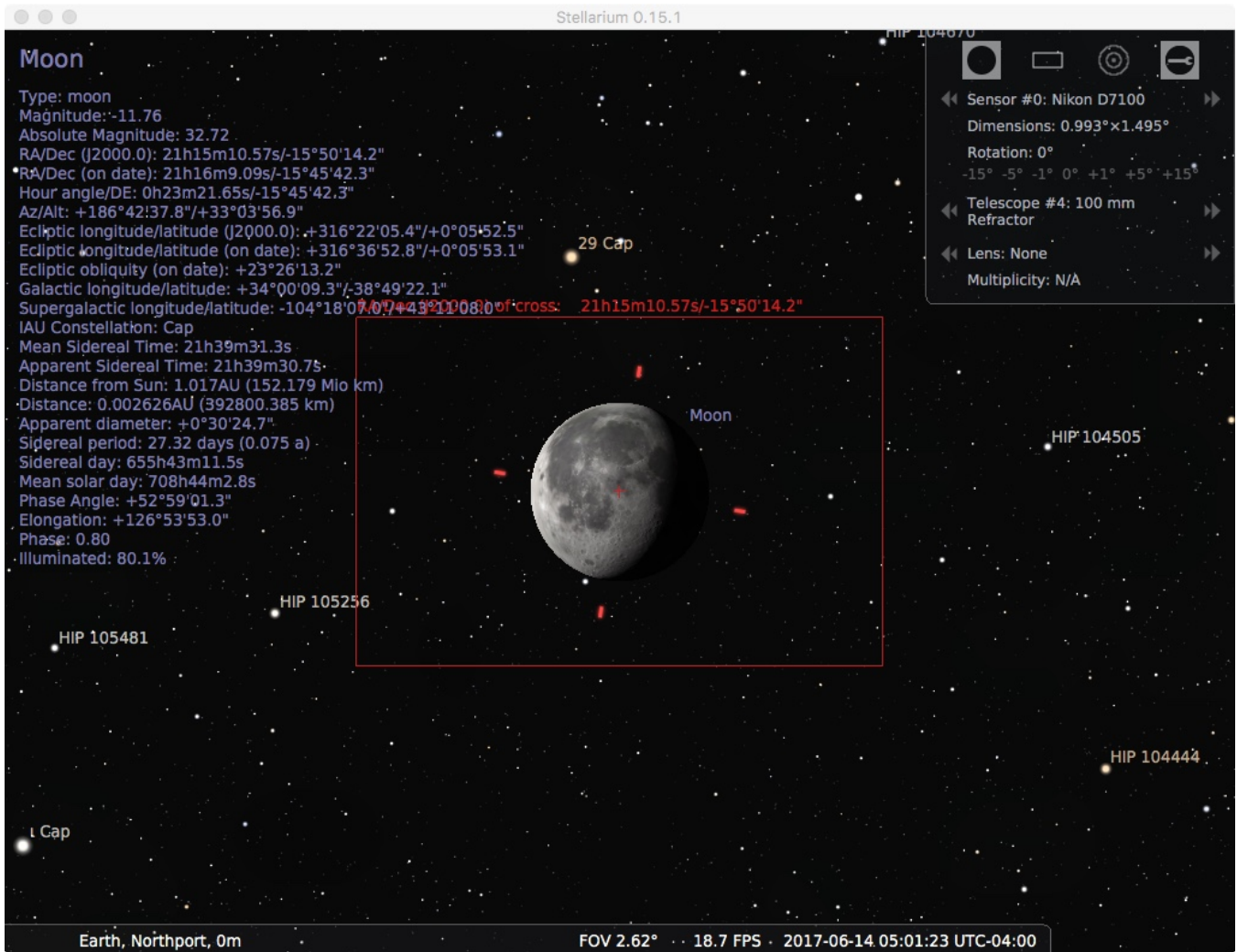
Moon - APS-C, 900 mm FL Telescope
