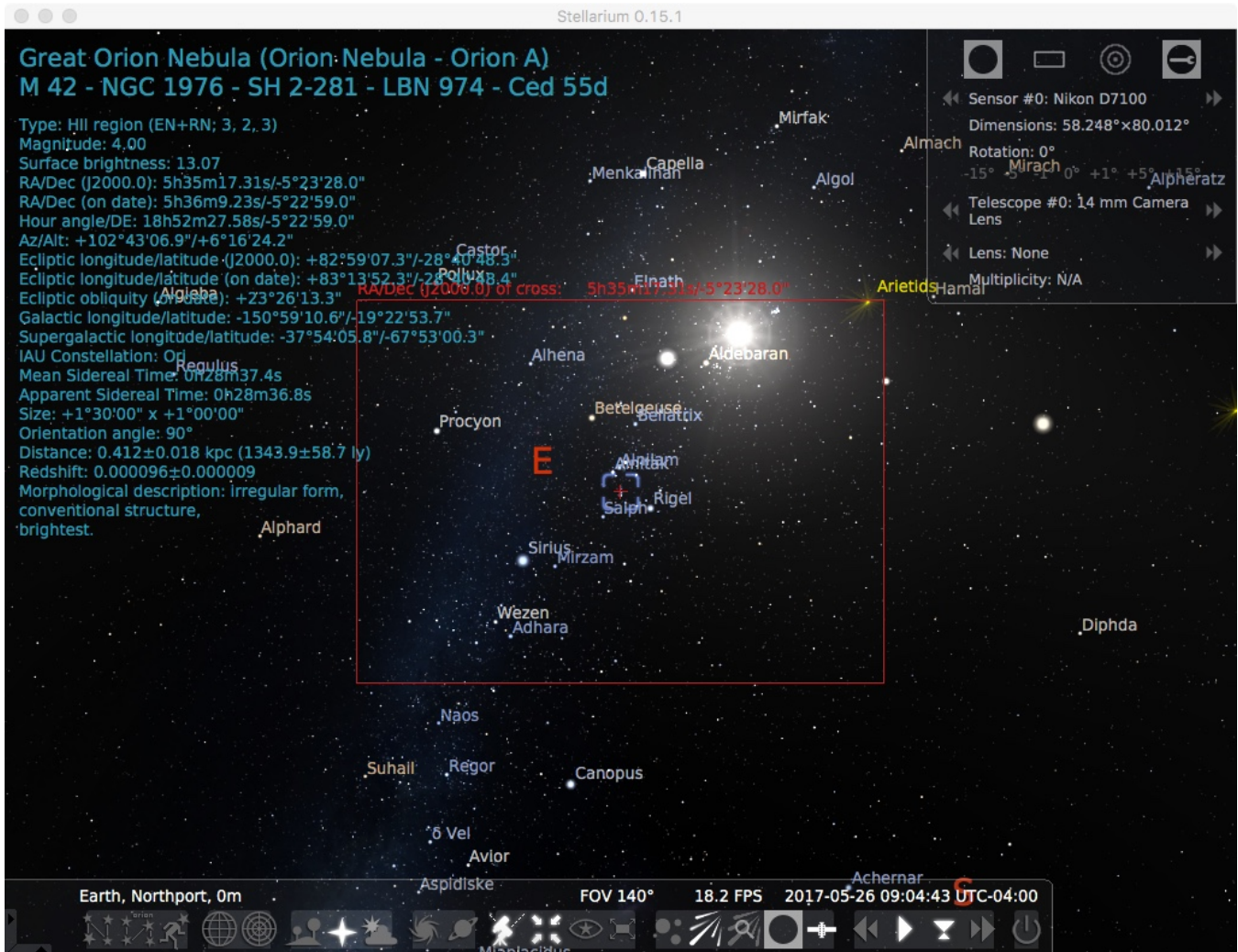
Orion Nebula - APS-C, 14 mm FL Lens
