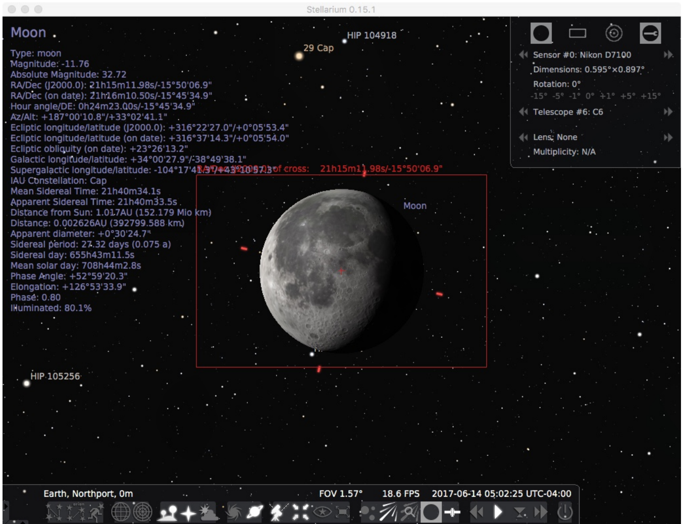
Moon - APS-C, 1500 mm FL Telescope
