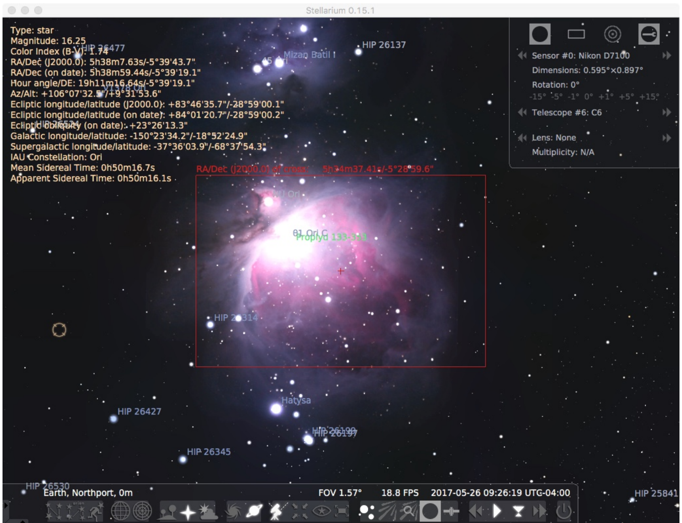
Orion Nebula - APS-C, 1500 mm FL Telescope
