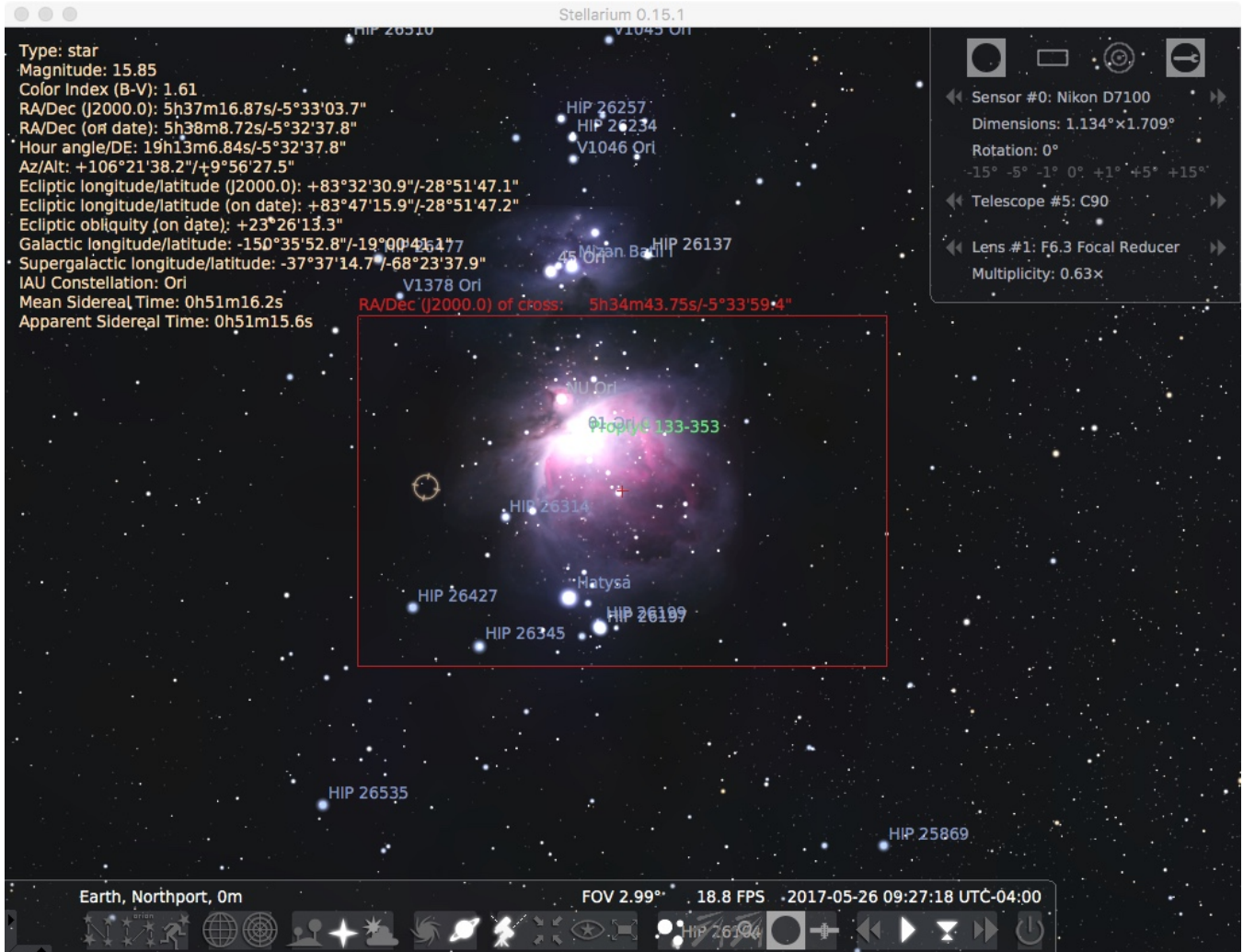
Orion Nebula - APS-C, 1250 mm FL FR.85 Telescope
