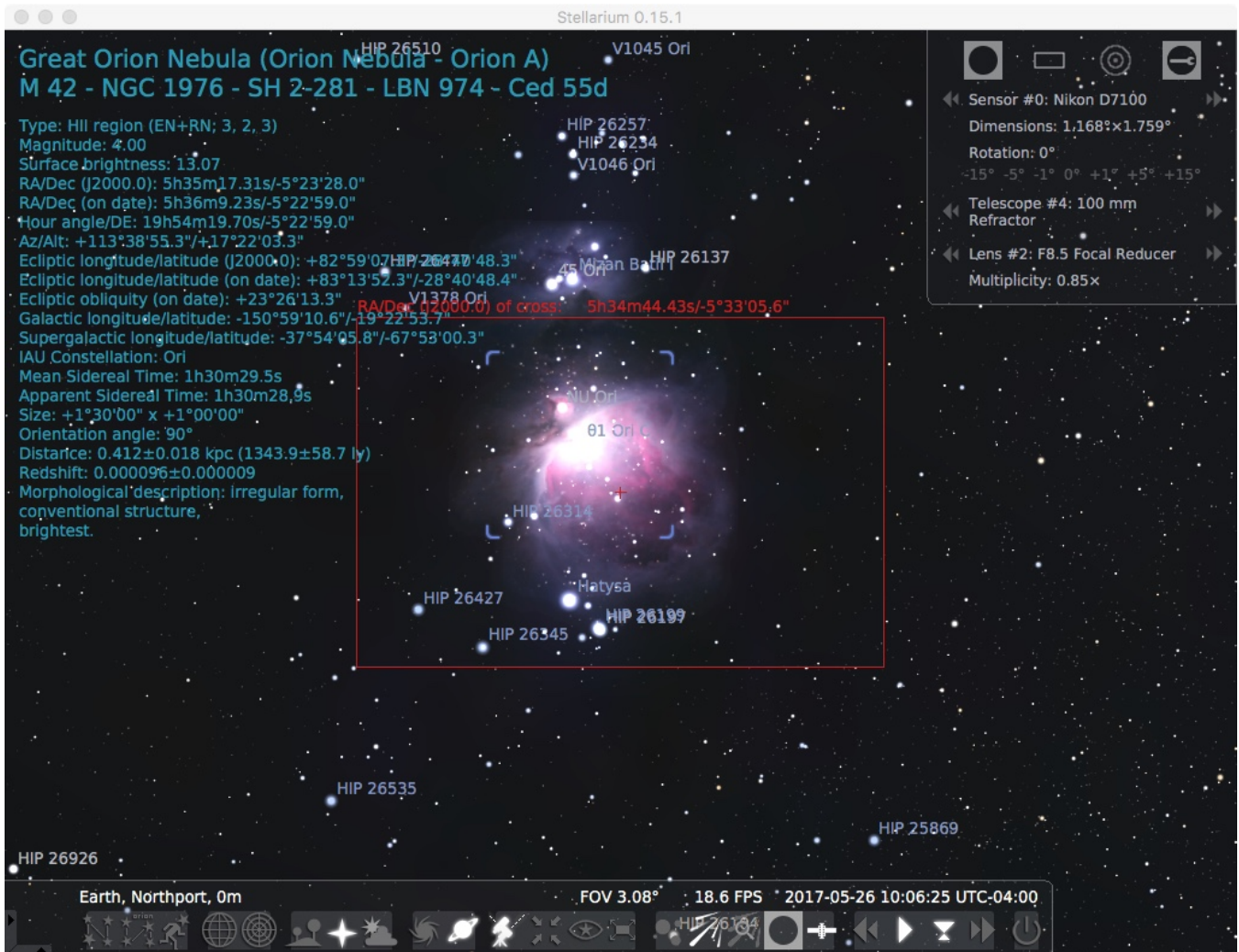
Orion Nebula - APS-C, 900 mm FL FR.85 Telescope
