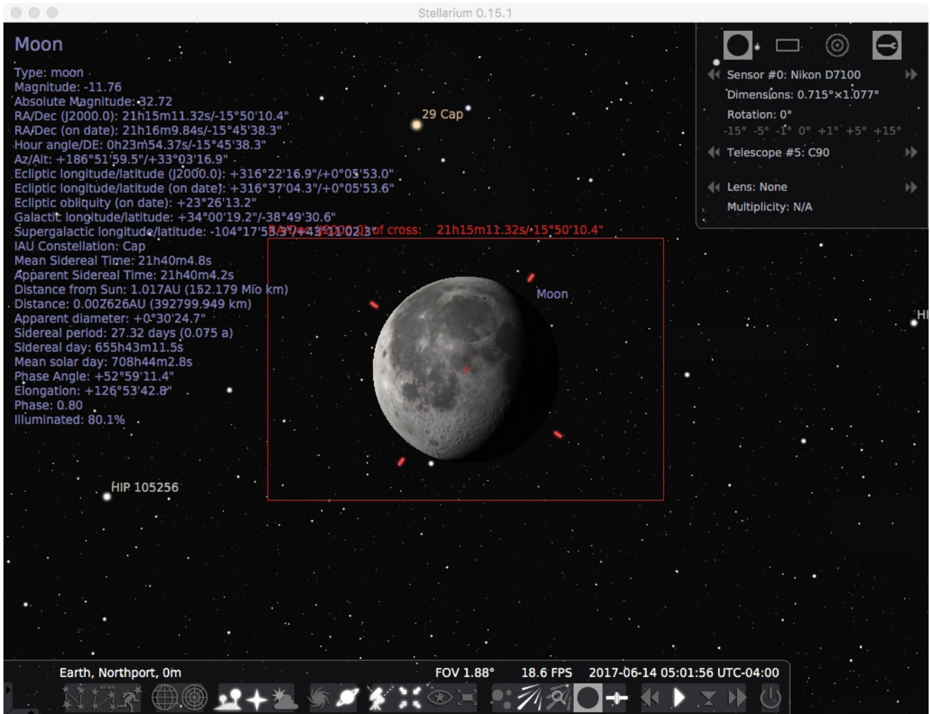
Moon - APS-C, 1250 mm FL Telescope
