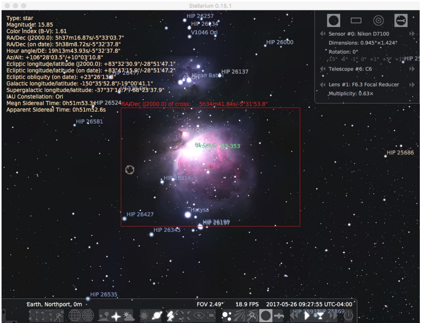
Orion Nebula - APS-C, 1500 mm FL FR.85 Telescope
