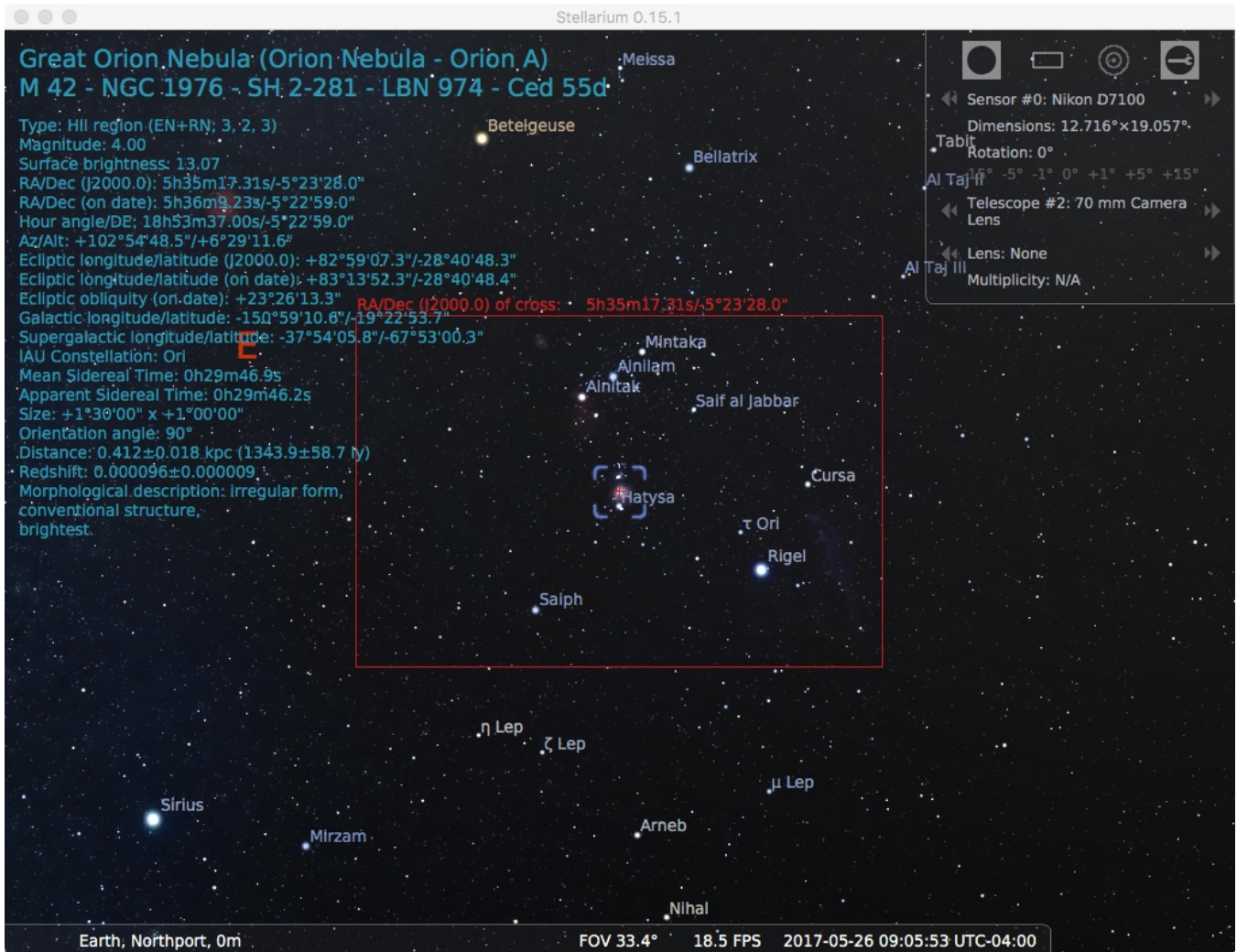
Orion Nebula - APS-C, 70 mm FL Lens
