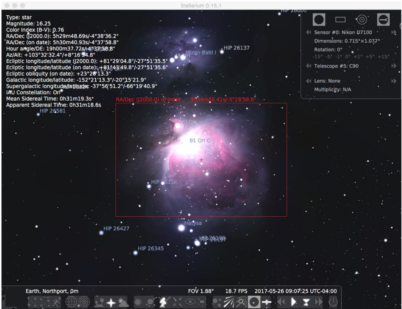
Orion Nebula - APS-C, 1250 mm FL Telescope
